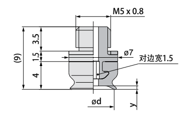
G-PTB02/B04/B06/08/15EU □ -H5
